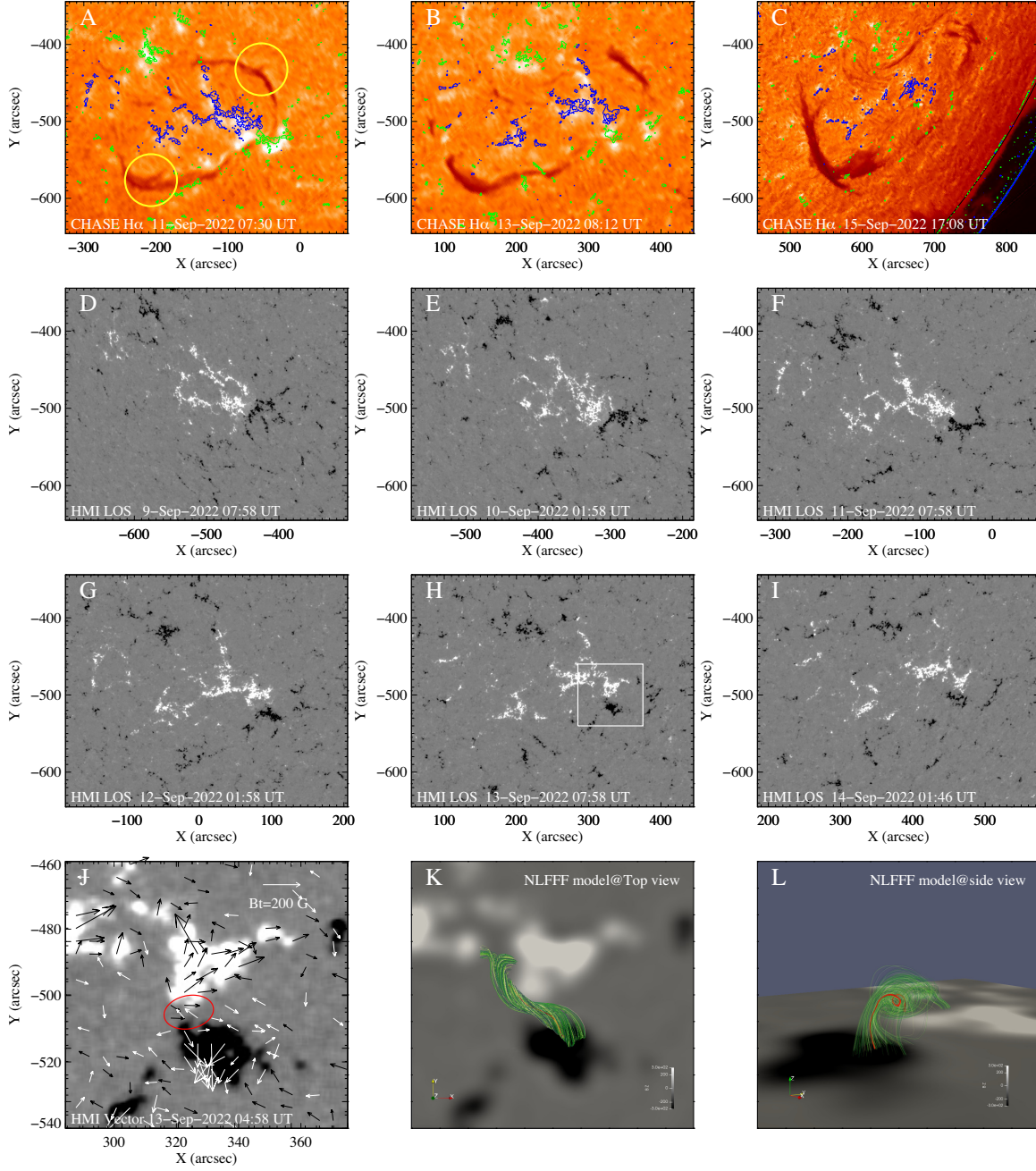
Figure A1. The long-term evolution of the filament channel, where mini- and giant filaments later erupt. (A-C) Selected H \alpha images taken by the CHASE, in which contours of simultaneous HMI magnetograms are overplotted at the level of \pm 300 Gauss. (D-I) HMI LOS magnetograms from 9 Sep 2022 to 14 Sep 2022. (J) HMI vector magnetogram in the region where minifilaments later form and erupt (see white rectangle in (H)). The black and white arrows represent the strength of positive and negative horizontal magnetic field, respectively. Red ellipse highlights one plausible bold patch in this region. (K) Top view and (L) side view of the NLFFF model over this region. The background is HMI magnetograms with the level of \pm 300 Gauss. In panel (L), one red line highlights the helical trend of field lines.
