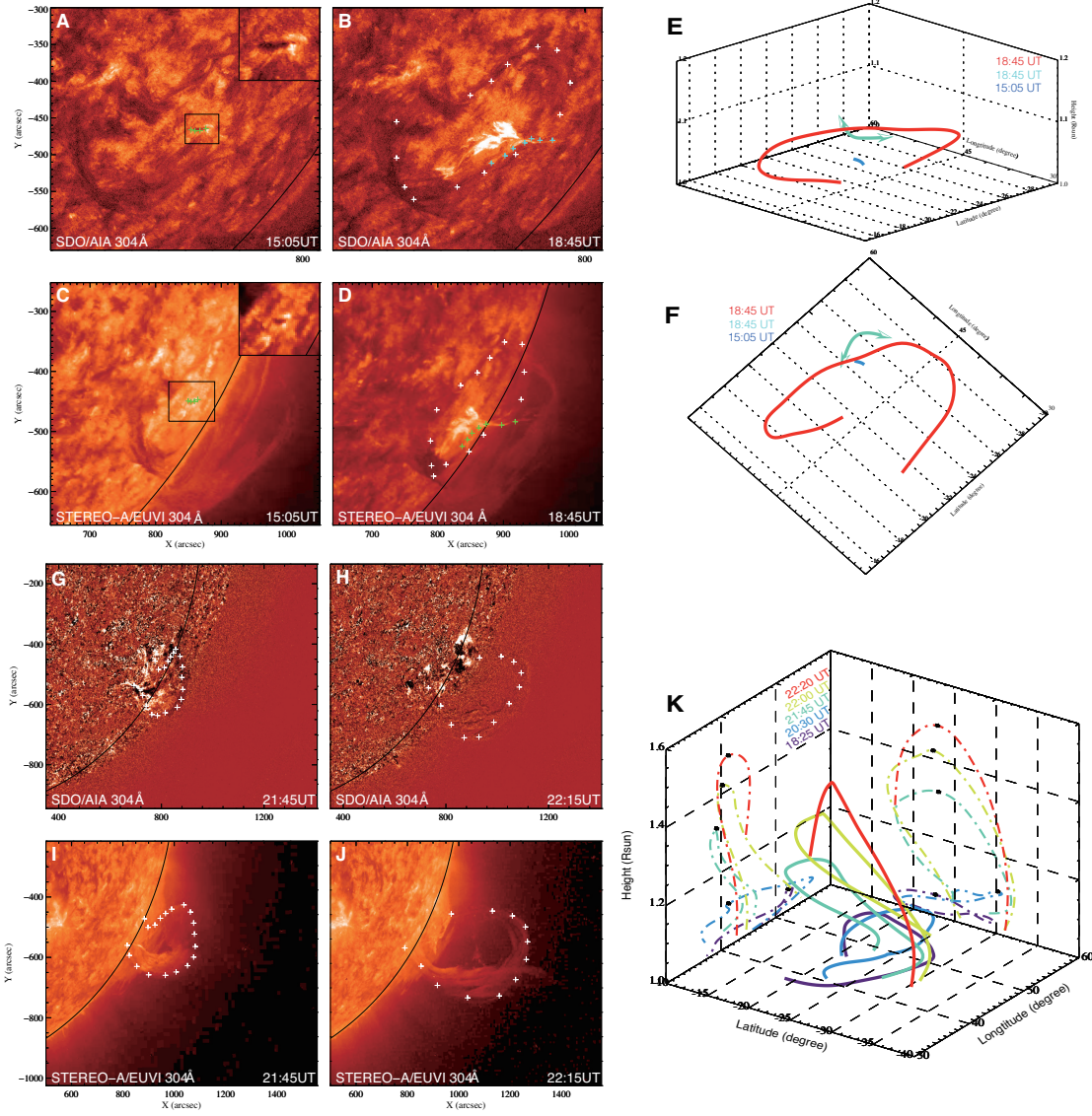
Figure A2. Three-dimensional reconstruction from dual-perspective SDO/AIA and STEREO-A/EUVI observations. (A-D) Dual-perspective snapshots of the third minifilament and the pre-eruption giant filament, as well as the two-side loop jets. A closed-up view of the minifilament is shown at the right-up corner of (A) and (C), respectively. (E-F) 3D reconstructed morphology of the pre-eruption giant (red curve) and miniature filaments (blue curve), as well as two-side loop jets (cyan curve), viewed from two different perspectives. (G-J) Dual-perspective snapshots of the erupting giant filament at two different times. (K) 3D reconstruction results of the erupting giant filament at different times, and their projections on two different 2D planes. The black asterisks indicate the top of filament main axis, respectively.
