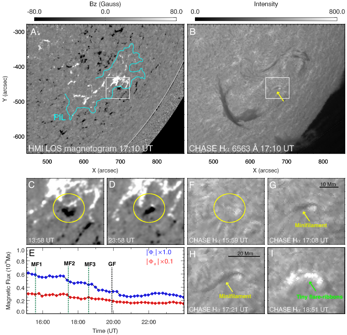
Figure 1. The formation and eruption of minifilaments underneath a giant filament due to small-scale flux cancellation on September 15th. (A) The SDO/HMI LOS magnetogram at 17:10 UT. The cyan solid line denotes the polarity inversion line (PIL) where both the minifilaments and giant filament form. (B) The CHASE H \alpha image at 6562.8 Å. (C-D) The convergence and cancellation of opposite-polarity small-scale magnetic flux concentrations. Another unrelated prominence is observed at the limb ( x = 730 , y = -600 ) and remains stable during the giant filament eruption. The field of view (FOV) is indicated by the white rectangle in (A). (E) Evolution of magnetic flux during 15:00–24:00 UT within the field of view (FOV) of (C). Four vertical dashed lines indicate the eruption times of three minifilaments (abbreviated as MF1, MF2, and MF3) and the overlying giant filament (abbreviated as GF), respectively. (F-I) Snapshots of minifilament activity in the FOV of (C). Features of interest are marked in each panel; see the text for details. An animation of panel (B) is available in the online journal. This animation presents a time sequence of 720 s LOS magnetograms and AIA 193 Å images spanning from 15:34 UT to 23:58 UT on 15 September 2022, with a total duration of 10 s.
