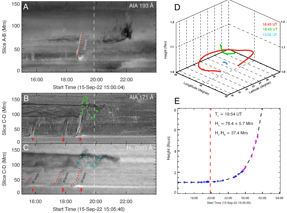
Figure 3. Eruptive dynamics and three-dimensional (3D) reconstruction of the giant filament. (A) Space-time diagram of AIA 193 Å images along slice AB in Fig 2A. The red dotted line highlights an upward-moving horizontal flux feature and its moving velocity is around 60 \text{ km s}^{-1} . (B-C) Space-time diagrams of AIA 171 Å and GONG H \alpha images along slice CD in Fig 2A, respectively. Three minifilament eruptions are marked by red numbers (1, 2, 3), respectively. Their velocity are fitted to be 37 \text{ km s}^{-1} , 30 \text{ km s}^{-1} , and 53 \text{ km s}^{-1} , respectively. The green/cyan diamonds highlight the plasma oscillation (amplitude \sim 50\text{--}70 \text{ Mm} ) of the giant filament near its south part. (D) The 3D morphology of minifilament (blue), giant filament (red), and two-sided loop jets (green) reconstructed through stereoscopic observations of STEREO-A/EUVI and SDO/AIA in 304 Å passbands. (E) Height of the main axis top of the erupting giant filament as a function of time and its fitting result (black dashed line). The blue dots represent stereoscopic measurements from SDO/AIA and STEREO/EUVI, and the purple dots are measured from LASCO/C2. The white dashed lines in (A-C) and the red dashed line in (E) indicate the fitted onset time (19:54 UT) of the giant filament eruption.
