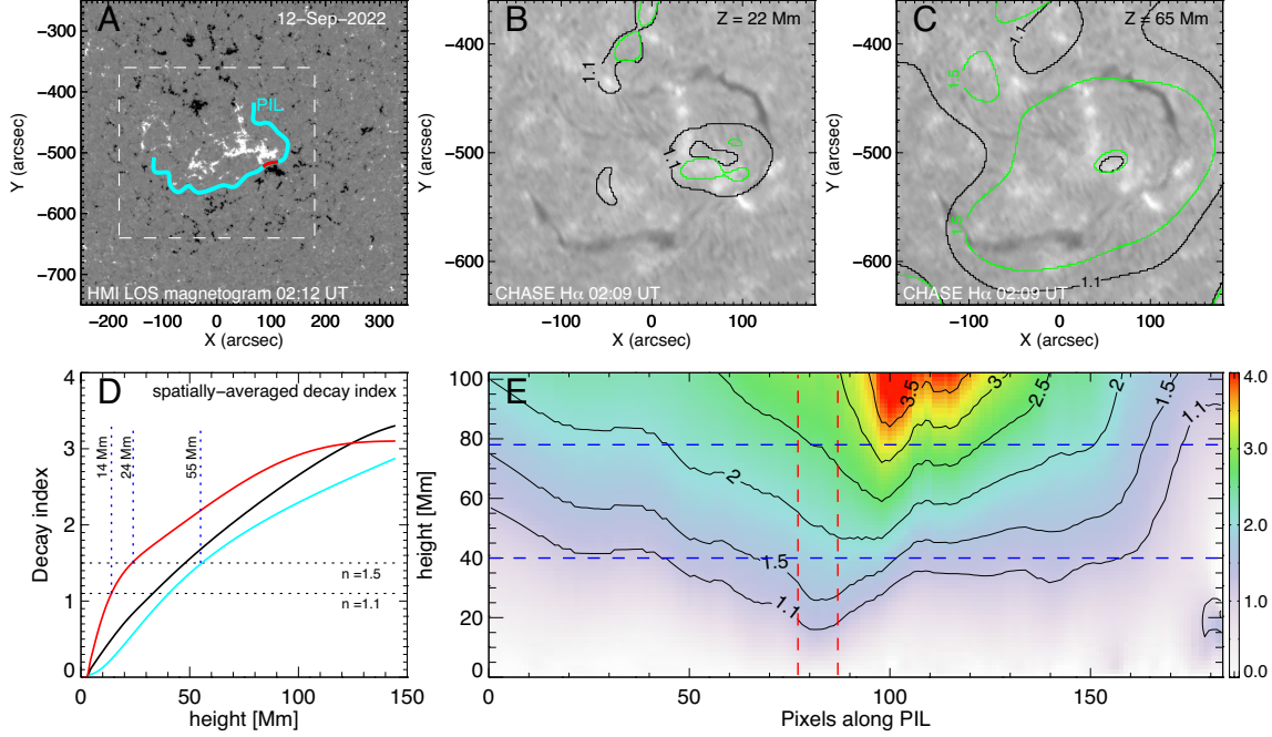
Figure 4. Magnetic decay index analysis above the PIL of miniature and giant filaments on 2022 September 12th. (A) Magnetic environment of the source region, as it passed the central meridian on 2022 Sep 12. Polarity inversion lines (PILs) of the whole filament channel and of the minifilaments are outlined by the cyan and red lines, respectively. (B) and (C): Two-dimensional spatial distributions of decay index at the heights of 22 Mm and 65 Mm are plotted over a simultaneously taken CHASE H \alpha image, respectively. (D) Spatially-averaged decay index as a function of height, which respectively are calculated over the whole PIL, the minifilament-related PIL (red section in (A)), as well as the rest PIL (two cyan sections in (A)). (E) The height variation of decay index above the whole PIL at 02:12 UT, in which contours at different levels are also plotted. Two red dashed vertical lines highlight the corresponding spatial range right above the PIL of minifilaments. Two blue dashed horizontal lines indicate the initial and maximum heights of the pre-eruption giant filament.
