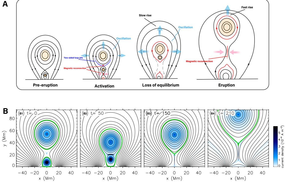
Figure 5. Two-dimensional schematic view and 2.5-D MHD simulation of the coupling between miniature and giant filament eruptions. (A) In the pre-eruption phase, a mini-MFR and a giant MFR are both at the equilibrium state in the same filament channel, forming a double-decker system. In the activation phase, homologous mini MFRs sequentially lose equilibrium and erupt towards the overlying giant MFR, leading to the activation of the giant MFR. In this course, multiple magnetic interaction occurs between magnetic field of the erupting mini MFR and overlying giant MFR, including magnetic reconnection and flux feeding (or axial magnetic field merging), as well as oscillation. Reconnection occurs both ahead and behind the erupting mini MFR, which leads to the two-sided loop jets and tiny standard flare arcades, respectively. In the loss-of-equilibrium phase, the flux merging process between mini- and giant MFRs facilitates the disruption of the whole system. In the eruption phase, a newly formed large flux rope becomes globally unstable and steps into its final eruption. (B) 2.5-dimensional MHD simulation reproducing the interaction, flux merging, oscillation, and the whole eruption of this double-decker MFR system. (B1) An initial double-decker flux-rope system with an HFT configuration. (B2) The flux merging between a small and a large flux rope and subsequent flux rope oscillation. (B3) The ascent of the newborn flux rope; (B4) The eruption of the newborn flux rope. The times indicated in panels (B1)–(B4) are in unit of \tau_A . The blue color depicts the distribution of the current density. The green curves indicate the boundary of the big and small flux ropes. An animation of Panel (B) is available in the online journal, depicting the 2.5D MHD simulation results. The duration of the animation is 13 s.
