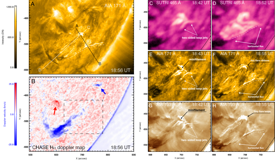
Figure 2. Magnetic interaction between the erupting minifilament and the overlying giant filament during the period from 18:30 UT to 19:30 UT on 2022 Sep 15. (A) The AIA 171 Å image at 18:56 UT. The solid lines AB (in black) and CD (in white) indicate the slice positions for the two space-time diagrams in Fig.4, respectively. The white dashed line outlines a bundle of upward-moving horizontal magnetic field or flux. (B) The Doppler map reconstructed from the CHASE H \alpha spectroscopic observation at 18:56 UT. Red/Blue arrow marks the redshift/blueshift at the left/right feet of the erupting giant filament, respectively. The black dashed rectangle represents the FOV of (C-H). (C-H) Zoom-in snapshots of the magnetic interaction process in SUTRI 465 Å, AIA 171 Å, and AIA 193 Å images. Features of interest are marked in each panel; see the text for details. An animation of this figure is available in the online journal, showing the interaction between the erupting minifilament and the giant filament. The duration of the animation is 3 s.
