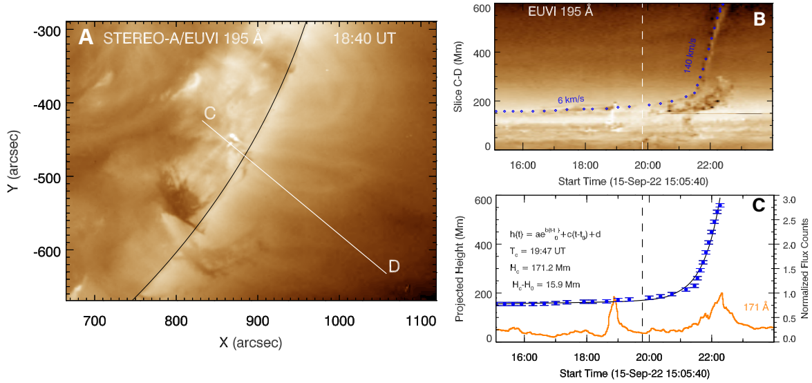
Figure A3. The eruption of the giant filament and its height-time evolution observed from the perspective of STEREO-A on 15 September 2022. (A) The STEREO-A/EUVI 195 Å image at 18:40 UT. The Slice CD represents the radial eruption path of the giant filament. (B) The space-time diagram along slice CD, showing the height-time evolution of the giant filament eruption. (C) The height-time profile of the erupting giant filament and its fitting result. The AIA 171 Å flux variation computed in the source region (see the same FOV of Fig. 3E) is also plotted. An animation of this Figure is available in the online journal. The animation begins before the time sequence shown in panel (A), with the EUVI 195 Å images (panel (A)) spanning from 15 September 2022 15:00 UT to 23:55 UT. The duration of the animation is 4 s.
